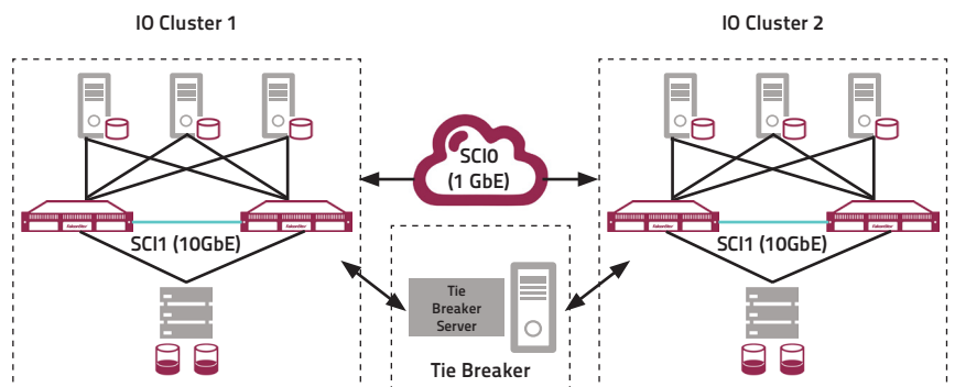
IO Multi-Cluster - "4-Way"
